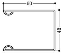
ROLLER GUIDE WITH ONE SILENCING STRIP
