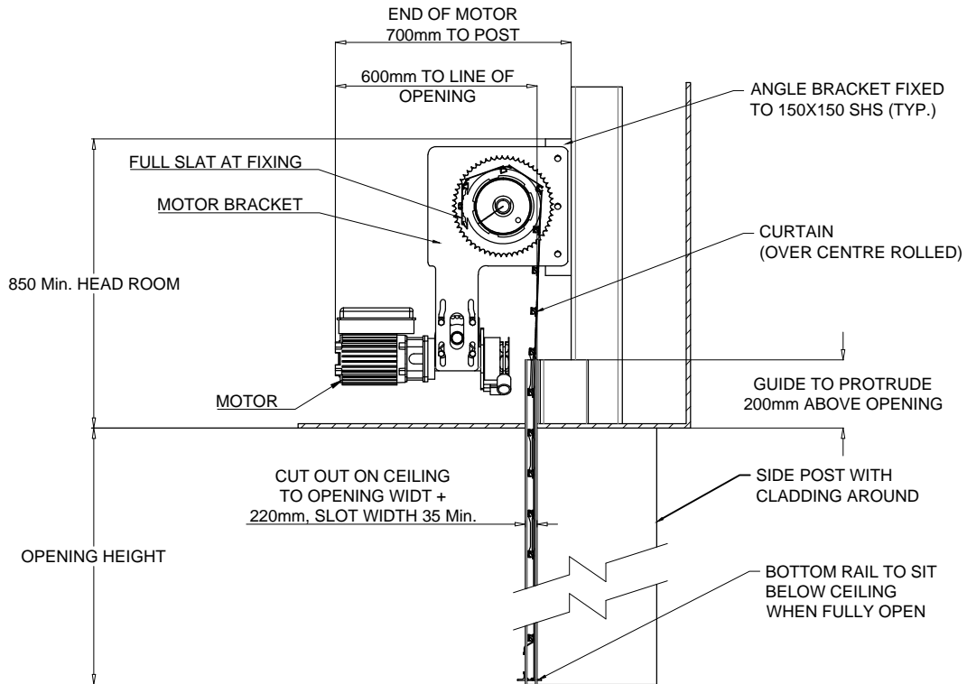
SECTION C-C
