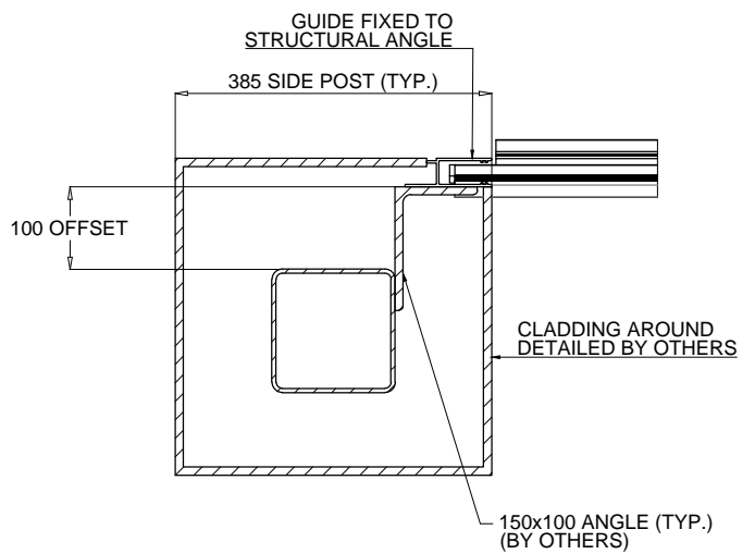
DETAIL E
